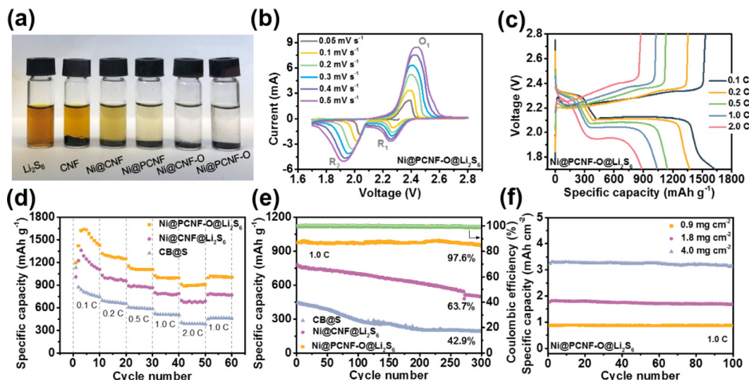
Fig. 5. LiPSs immobilization of Ni@PCNF-O composite: (a) Digital photographs of different samples after static adsorption of \text{Li}_2\text{S}_6 . (b) CV curves under different scanning rates, and (c) Voltage profiles at various current densities of Ni@PCNF-O@ \text{Li}_2\text{S}_6 half-cell. (d) Rate capabilities and (e) long-term cycling stability at 1.0 C of different half-cells. (f) Cycling performance of the Ni@PCNF-O@ \text{Li}_2\text{S}_6 half-cells with different sulfur loadings at 1.0 C.
