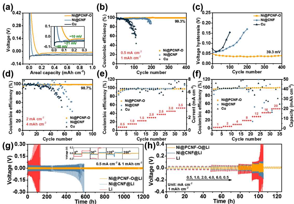
Fig. 4. (a) Voltage profiles of Li plating on different electrodes at 0.5 mA cm -2 . The inset shows the magnified nucleation overpotentials. (b) CE and (c) the corresponding voltage hysteresis of different electrodes at 0.5 mA cm -2 with the plating capacity of 1 mAh cm -2 . (d) CE profiles at 2 mA cm -2 with 4 mAh cm -2 . CE of different electrodes with increasing (e) current density and (f) capacity. Comparisons of (g) cycling performance and (h) rate performance of different electrode based symmetrical cells.
